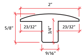
T-Molding 78" in Length
