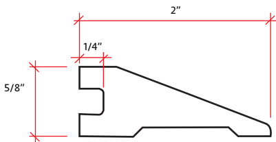
Reducer 78" in Length
