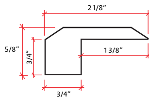
Threshold 78" in Length
